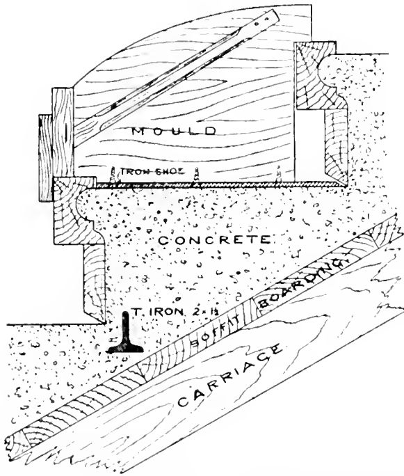
NO. 196.—SECTIONS OF FRAMING OF SOFFIT OF STAIR, RISER AND NOSING MOULD, WITH CONCRETE AND TREAD RUNNING MOULD IN POSITION.
